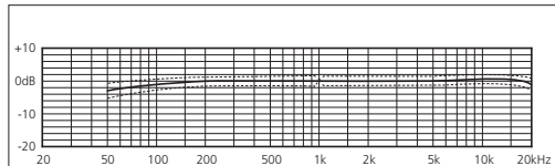
Frequency response curve MK 22 + CMC 6
